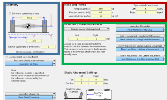
Figure 29: CarSim Rear Suspension Section
